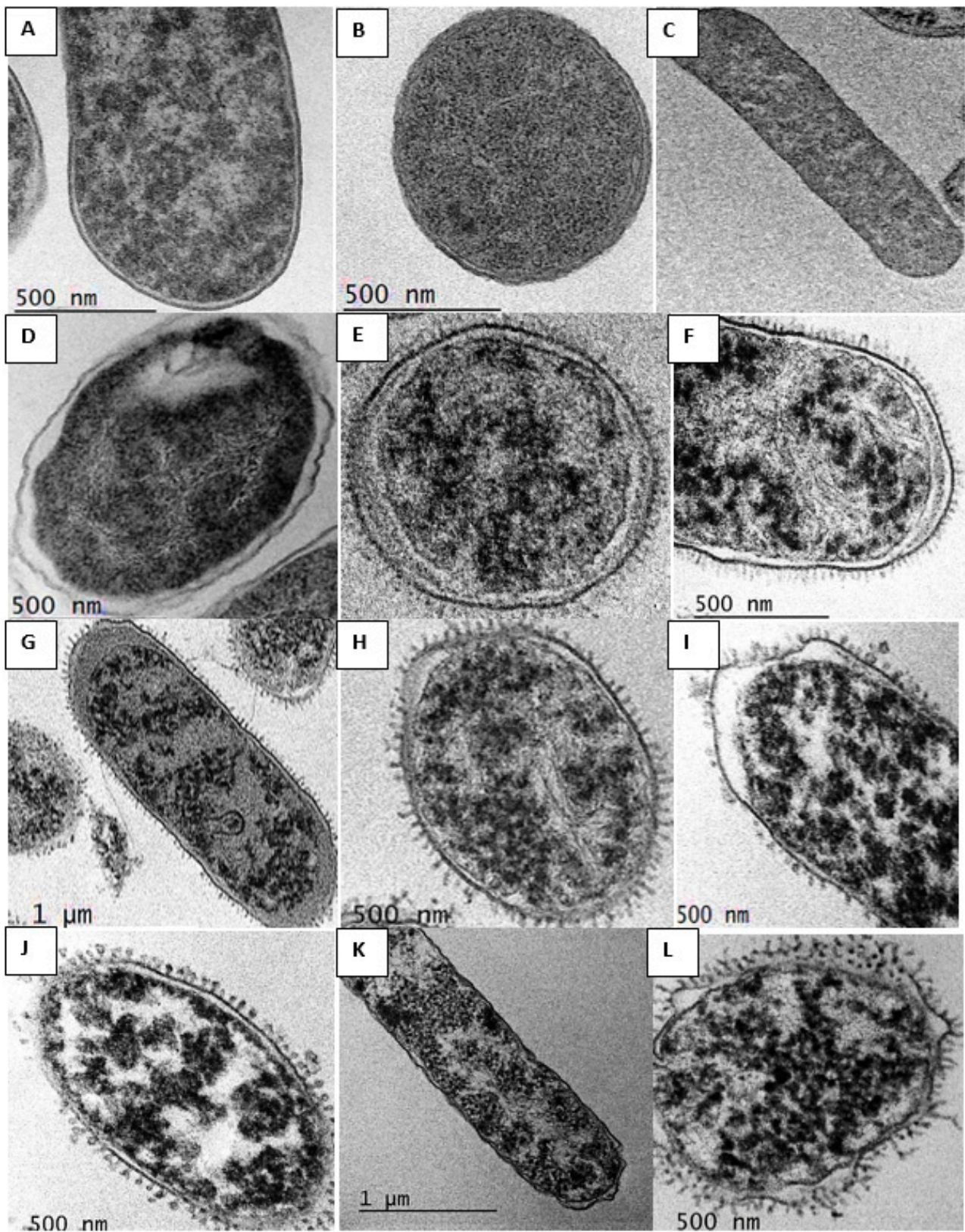
Figure 3. TEM micrographs of Escherichia coli 184 cells treated with (A–C) control; (D) Alg NPs (500 µg/mL); (E–F) Colistin (8 µg/mL); (G–H) Alg NPs+Colistin (500:1.25) µg/mL; (I–J) Alg NPs+Colistin+Lactic acid (500:0.62:15) µg/mL; (K–L) Alg NPs+Colistin+Menthol (500:0.31:10) µg/mL.
