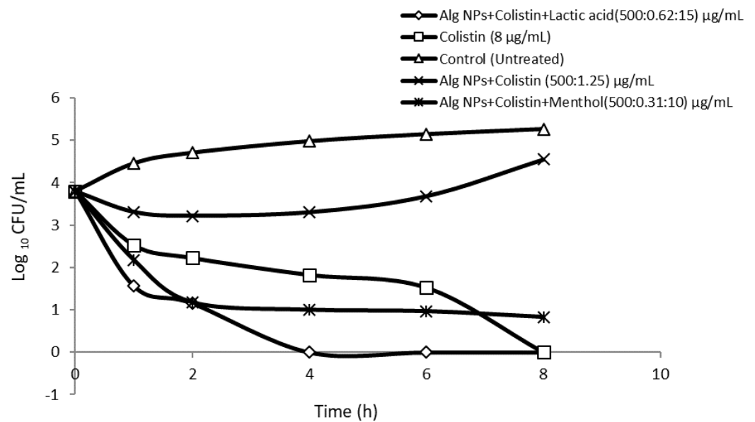
Figure 2. Killing curves of Escherichia coli 184 treated with different formulations of colistin associated with Alg NPs and menthol or lactic acid.
